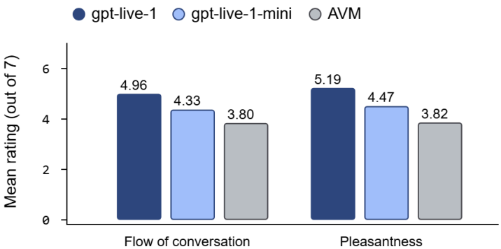
Model Conversation Ratings
